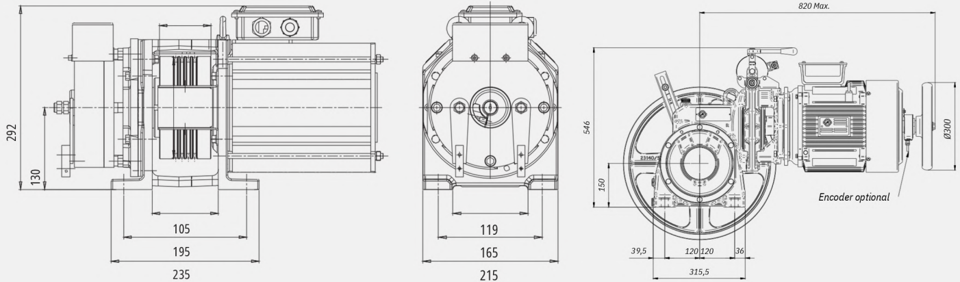
MOTOR TECHNICAL DRAWING
